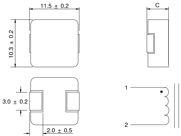
Dimensions(mm)
